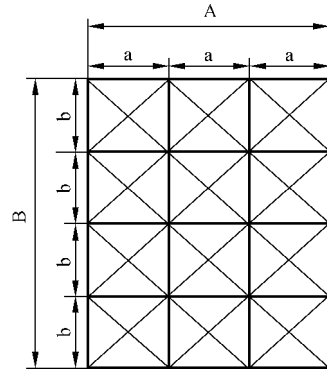
图 2 矩形风口测点布置
